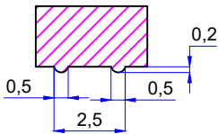
DETAIL-I GULF EXTRUSIONS (IDENTIFICATION MARK)
